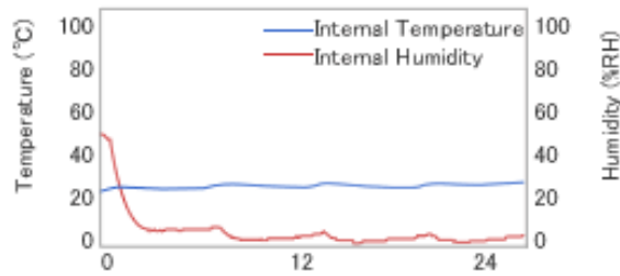
The variation of internal atmosphere within 24 hrs External atmosphere: 25°C, 50%RH
