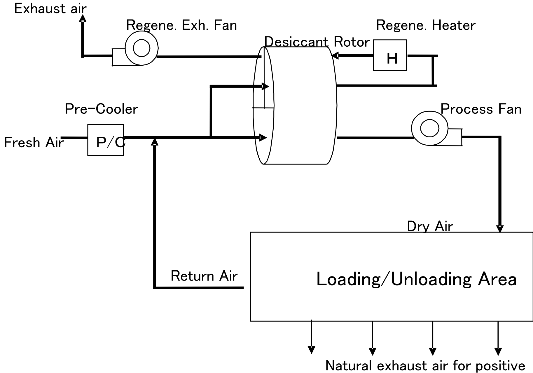
<Figure 1> Air Flow System
